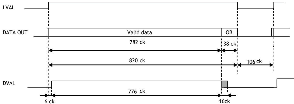
Fig.21. Horizontal Timing for Partial Scanning
