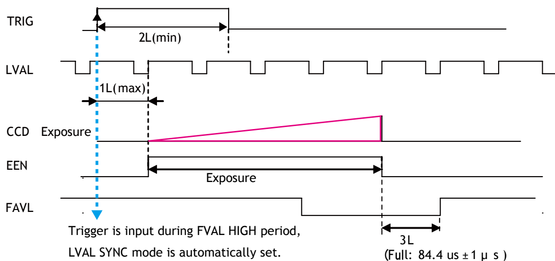
Fig. 24. Pre-select LVAL sync Timing
