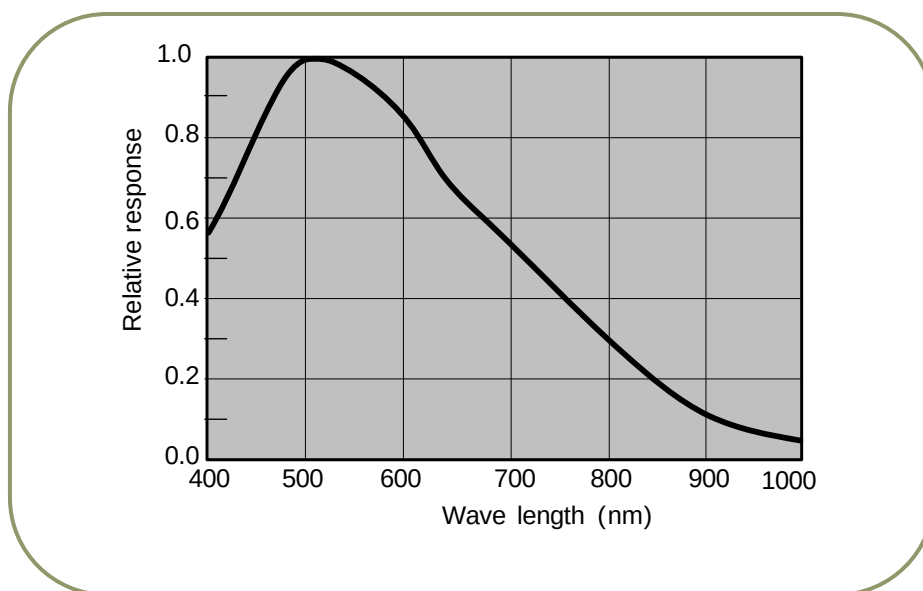
Fig. 29. Spectral response for CM-040GE
