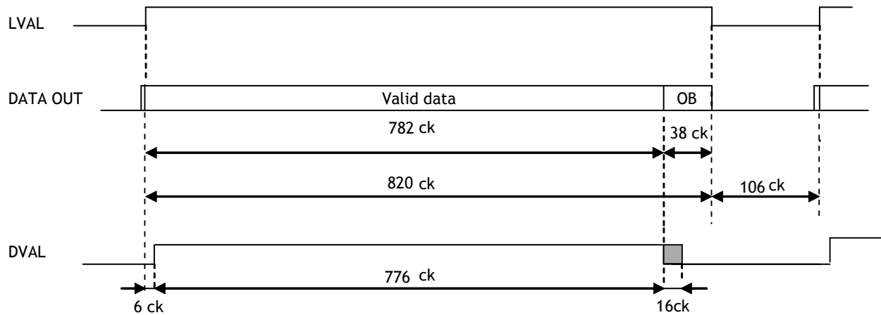
Fig. 18. Horizontal timing
