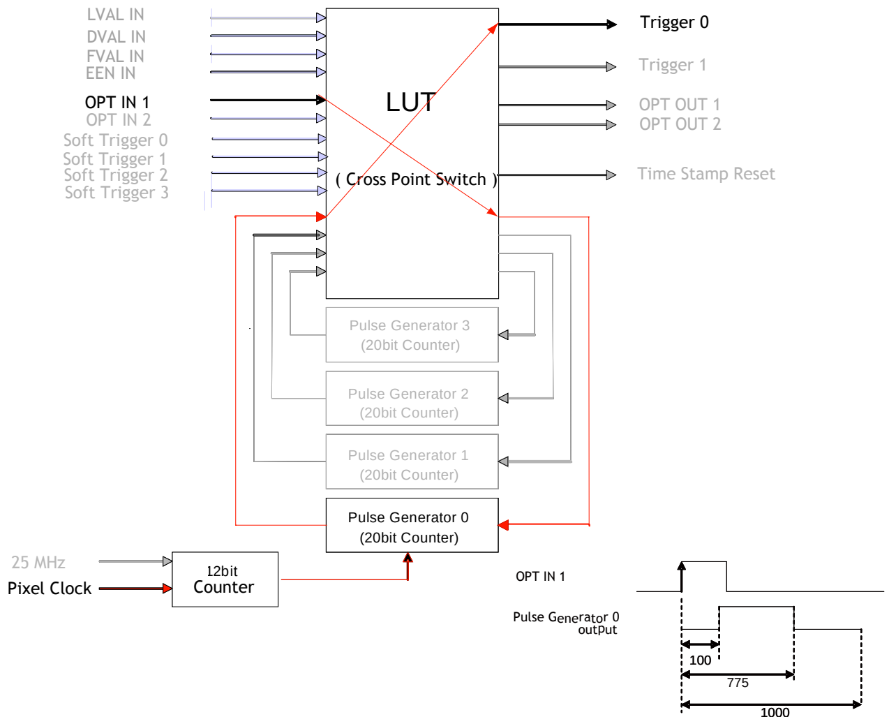
Fig.8. Pulse Generator Timing Example 1
