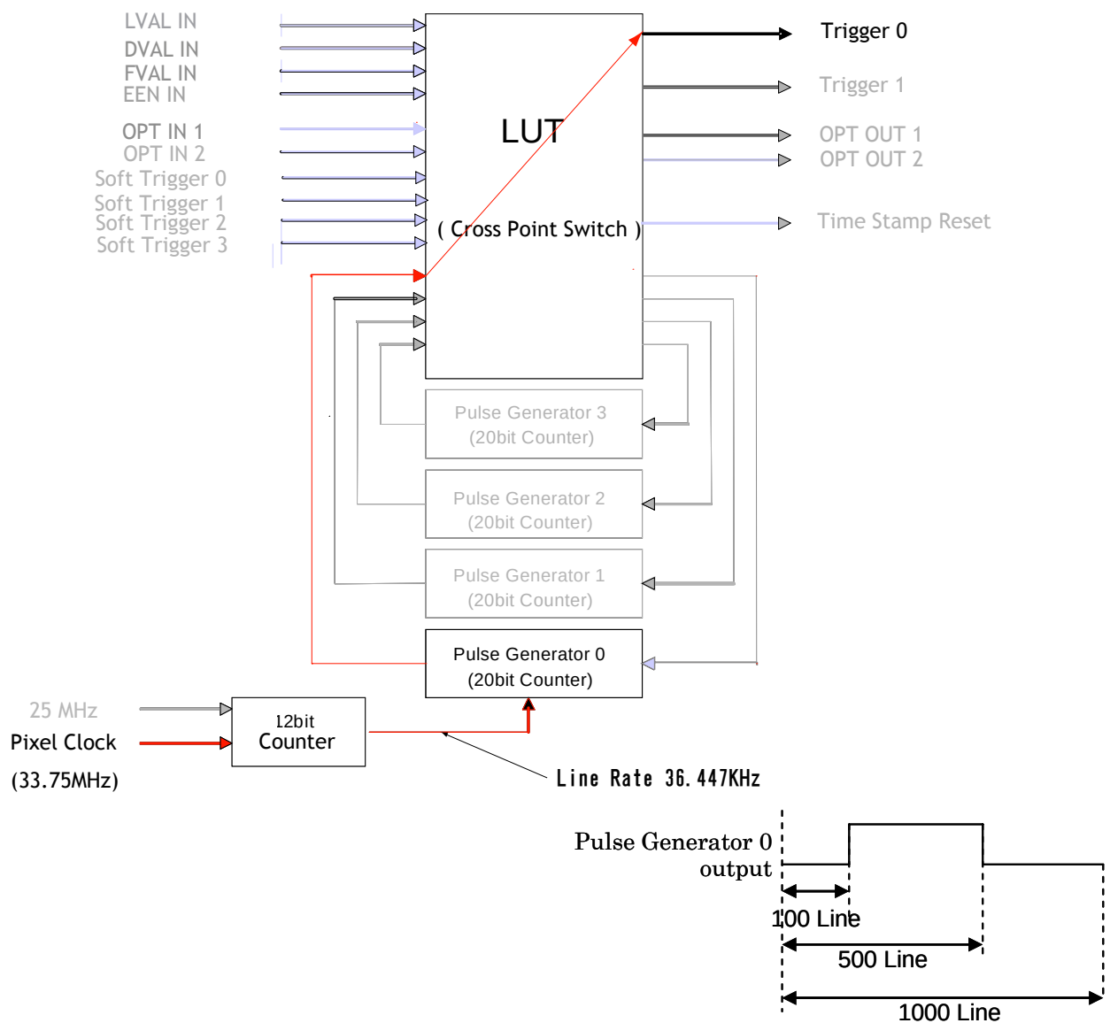
Fig.9. Pulse Generator 0 timing Example 2
