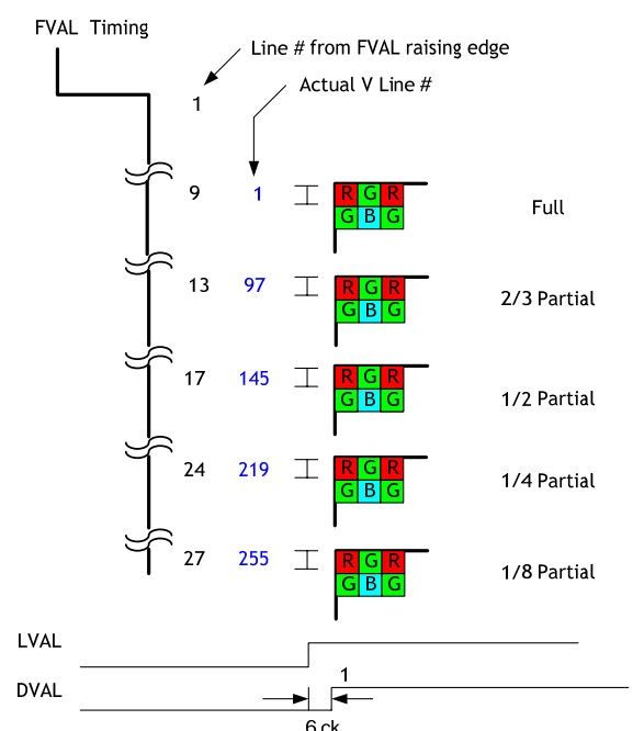
Fig.12. Bayer layout for each scan mode
