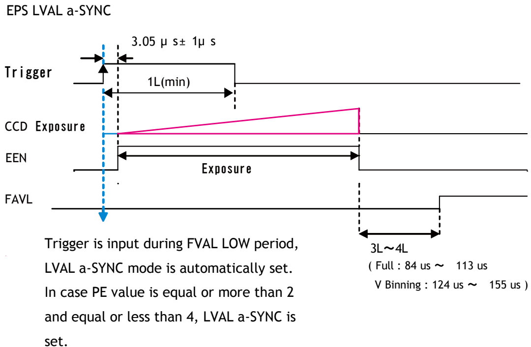
Fig.25. Pre-select LVAL async Timing
