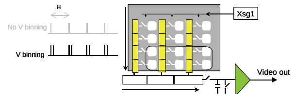
Fig.11. CM-040GE binning.
