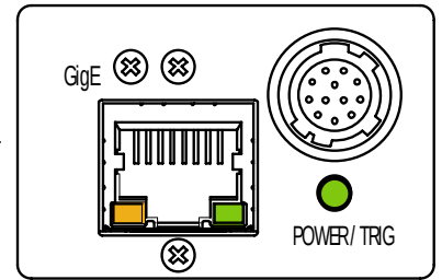
Fig.16. Rear Panel
