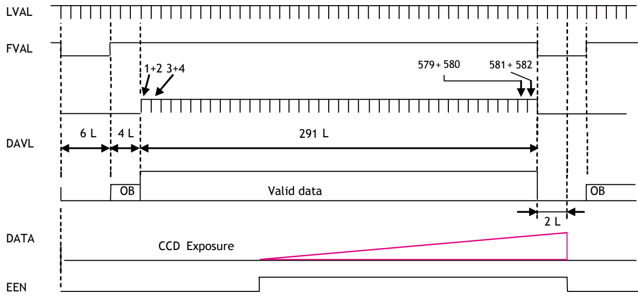
Fig.23. Vertical Timing for Vertical Binning
