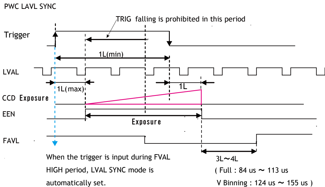
Fig. 26. Pulse width control. LVAL sync.
