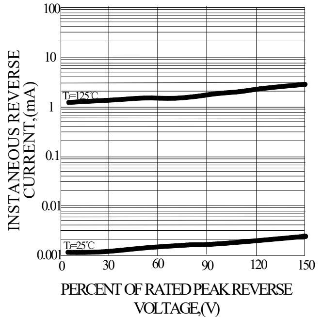
FIG.4-TYPICAL REVERSE CHARACTERISTICS
